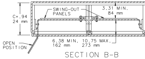
Showing four swing-out panels and center panel support mounted in two-door enclosure.
