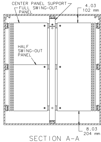
Showing swing-out panels installed in one-door enclosure.
